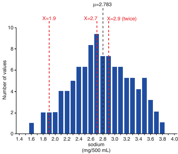
4.7 Random values from the example distribution figure
