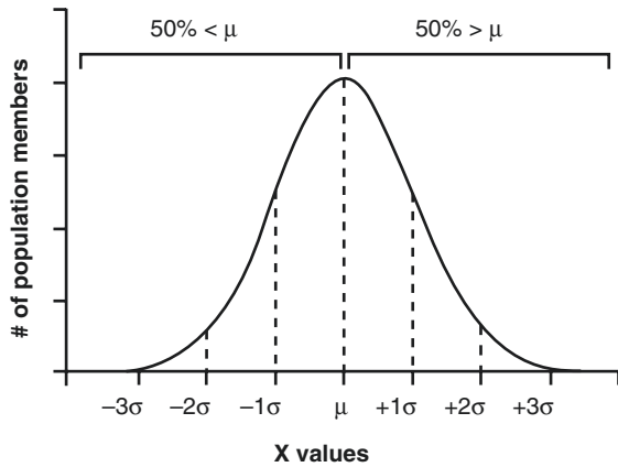
4.6 Densities of normal distributions figure
